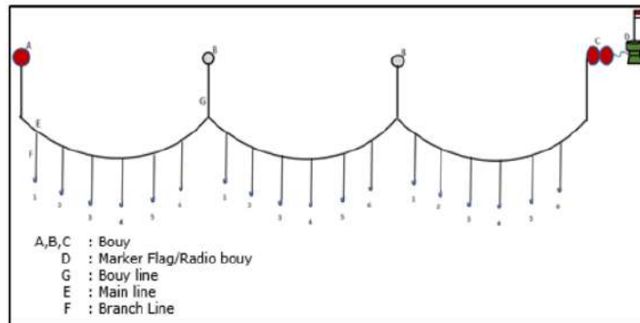
Figure 5. Sketch of basket with 6 branch lines.
