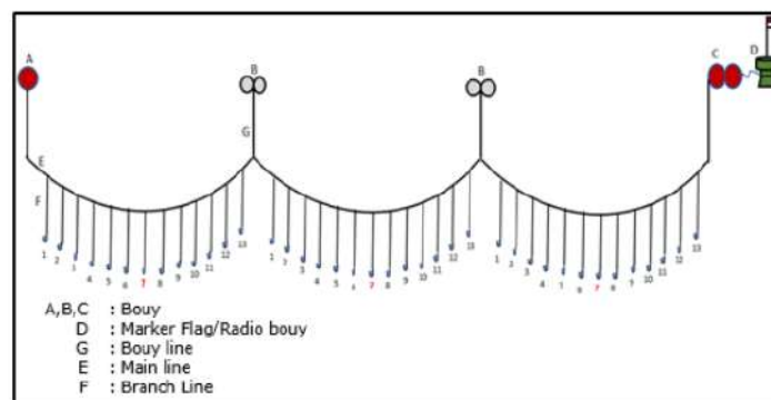
Figure 4. Sketch of basket with 13 branch lines.
