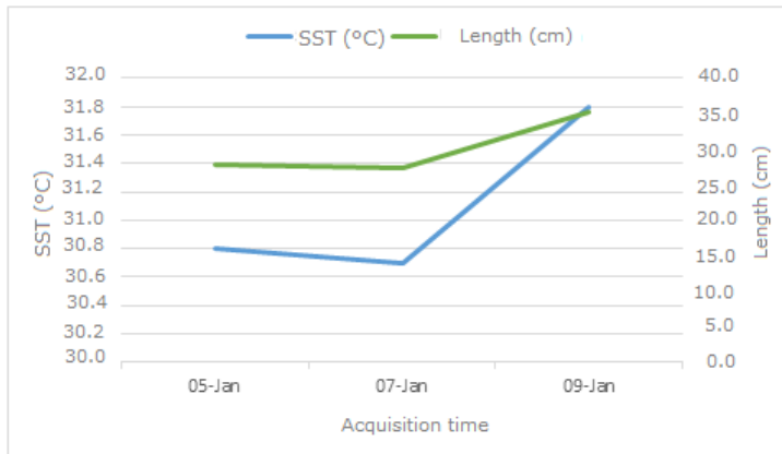
Figure 14. Relationship between SST and the length of K. pelamis in January 2018
