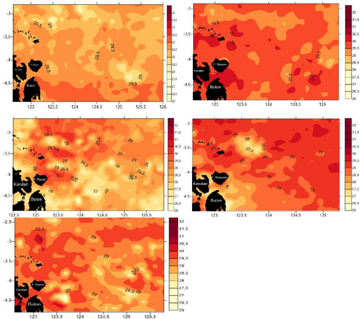
Figure 6. SST satellite imagery. a) November 2017 b) December 2017 c) January 2018 d) February 2018 and e) March 2018.
