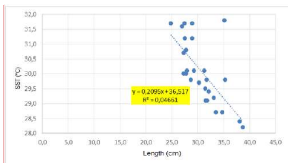
Figure 10. Relationship of SST with length size of Katsuwonus pelamis .
