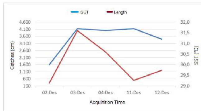
Figure 12. Relationship between SST and catch in December 2017 with a temperature range of 29°C to 31.5°C with catches of K. pelamis ranging from 300 kg to 4.000 kg.
