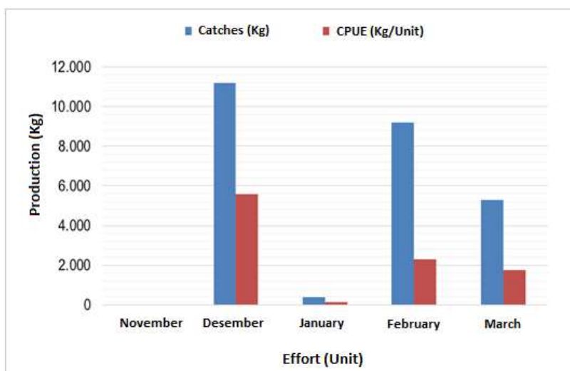
Figure 2. Amount of catch and CPUE in November, December, January, February, March 2018.
