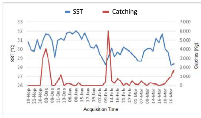
Figure 9. SST relationship with the catch of each setting.
