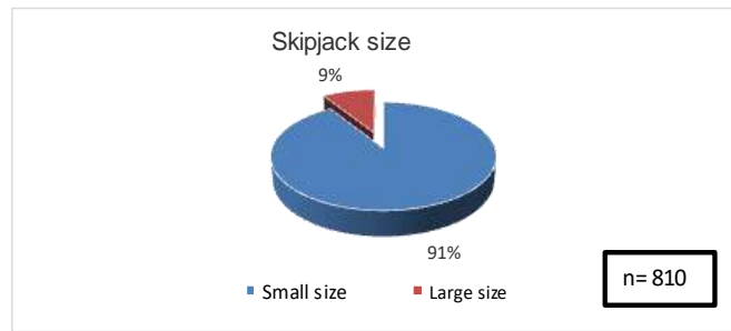
Figure 4. K. pelamis size in November 2017-March 2018.
