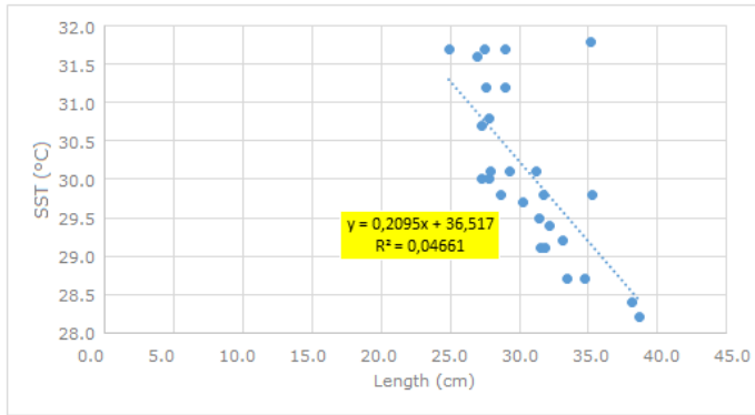
Figure 10. Relationship of SST with length size of K. pelamis .
