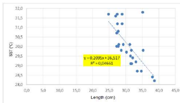
Figure 10. Relationship of SST with length size of K. pelamis
