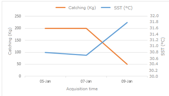
Figure 13. Relationship between SST and catching in January 2018
