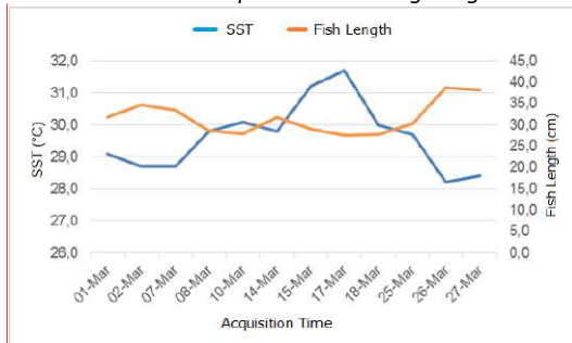
Figure 19. Relationship of SST with the length of Katsuwonus pelamis in March 2018 with a temperature range of 28.2-31.7°C and with a range of lengths of 27.5-38.7 cm.
