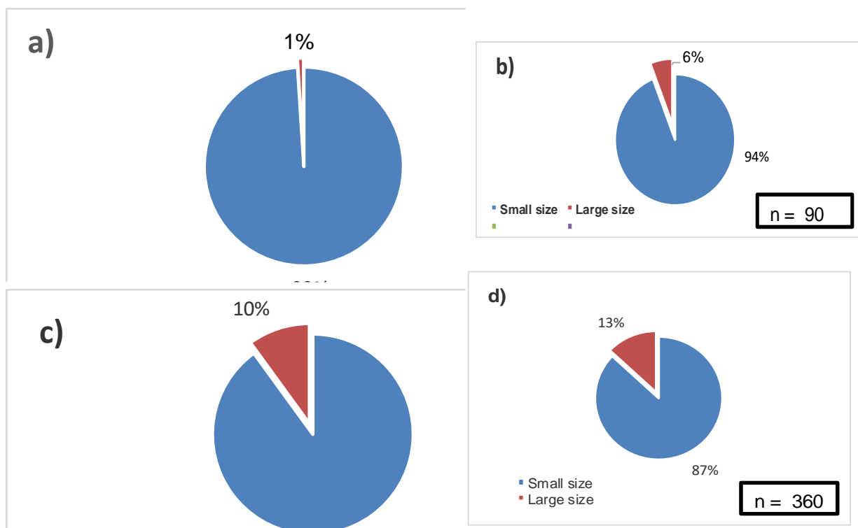
Figure 5. Monthly size of K. pelamis in months (a) December 2017 (b) January 2018, (c) February 2018, and (d) March 2018.
