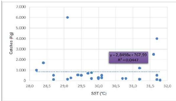
Figure 8. Relationship between SST and Katsuwonus pelamis catches.
