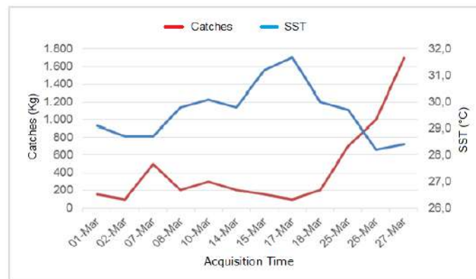
Figure 18. Relationship of SST and catches in March 2018 with a temperature range of 28.2°C to 31.7°C with K. pelamis catching a range of 100 kg to 1,700 kg.
