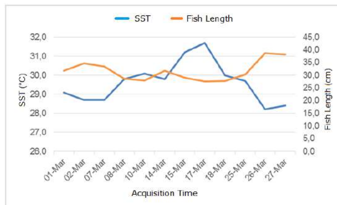
Figure 19. Relationship of SST with the length of K. pelamis in March 2018 with a temperature range of 28.2°C to 31.7°C and with a range of lengths of 27.5 cm to 38.7 cm.
