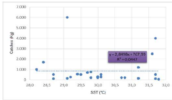
Figure 8. Relationship between SST and K. pelamis Catches
