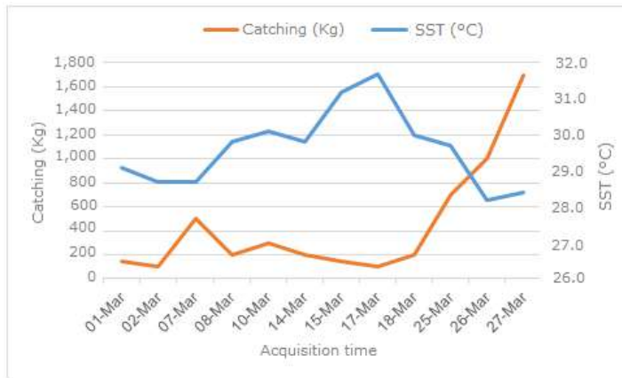
Figure 17. Relationship of SST and catches in March 2018
