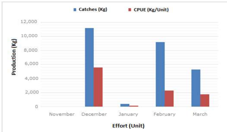
Figure 2. Amount of catch and CPUE in November, December, January, February and March 2018.
