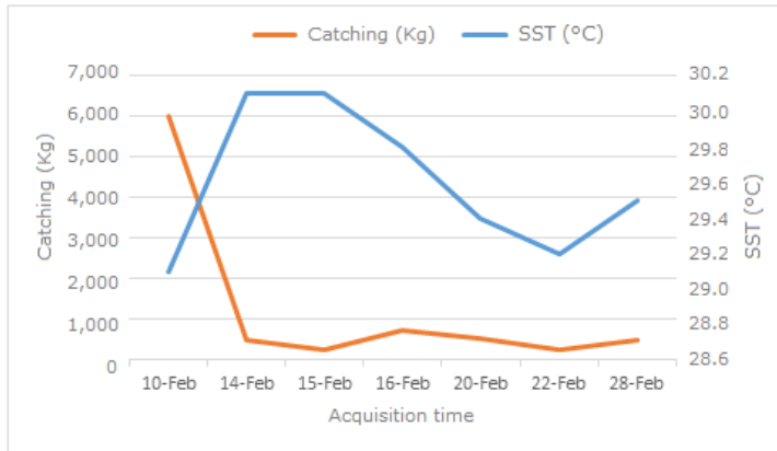
Figure 15. Relationship between SST and catching in February 2018 kg.
