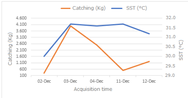
Figure 11. Relationship between SST and catching in December 2017
