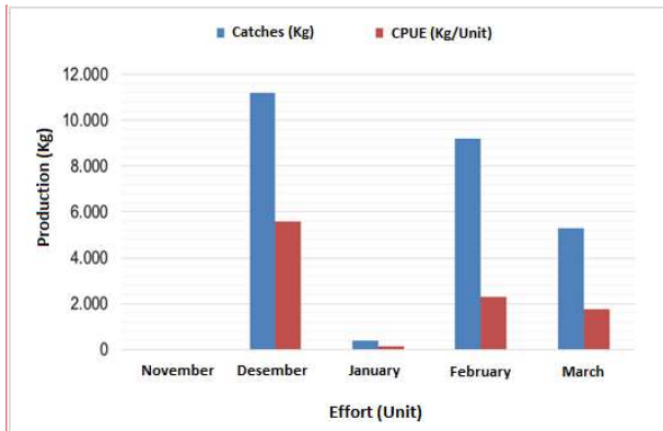
Figure 2. Amount of catch and CPUE in November, Desember, January, February, March 2018.
