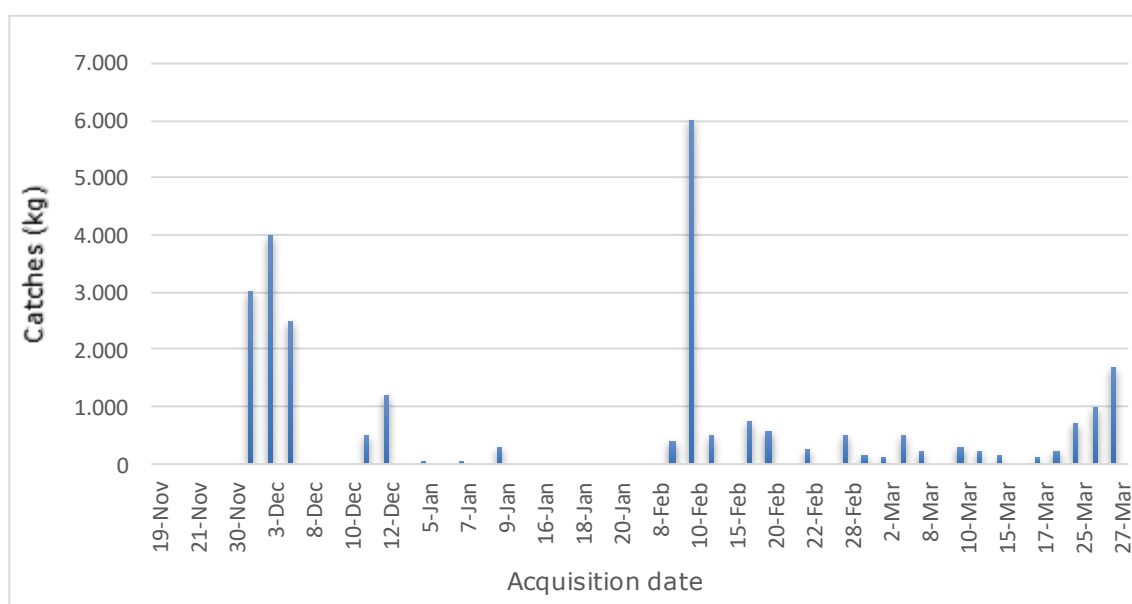
Figure 3. Daily catches in November, December, January, February, March 2018.
