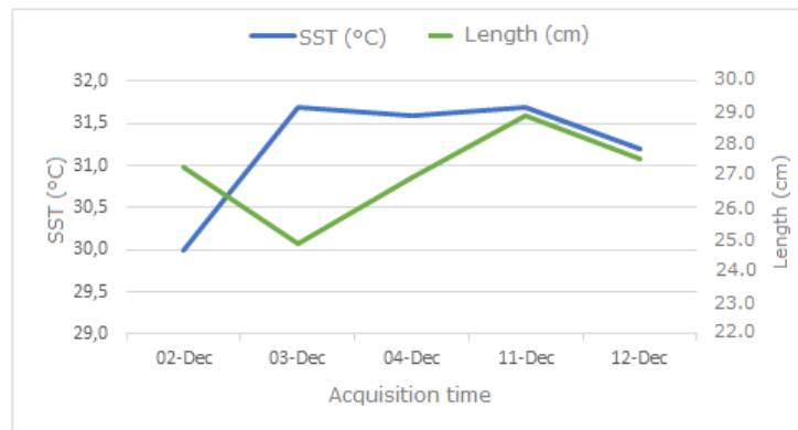
Figure 12. Relationship of SST with the length of K. pelamis in December 2017
