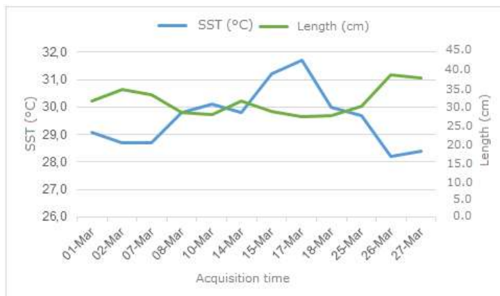
Figure 18. Relationship of SST with the length of K. pelamis in March 2018
