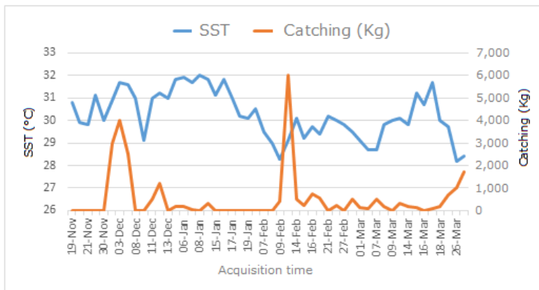
Figure 9. Sea Surface Temperature relationship with the catching of each setting.
