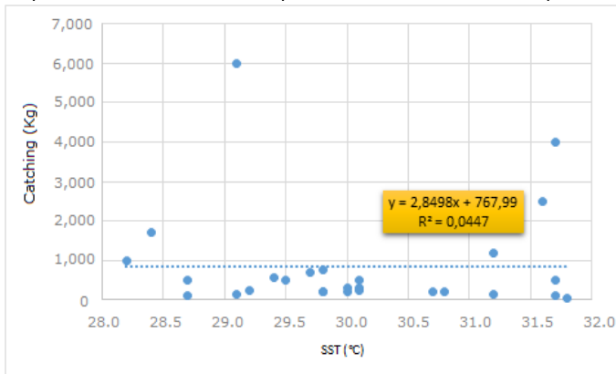
Figure 8. Relationship between Sea Surface Temperature and K. pelamis catches.
