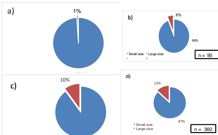
Figure 5. Monthly size of K. pelamis in (a) December 2017 (b) January 2018, (c) February 2018, and (d) March 2018.
