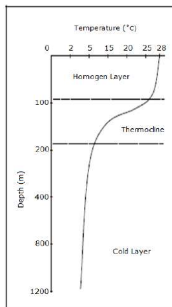
Figure 1. Changes in temperature at different sea depths. (Nontji, 1993).
