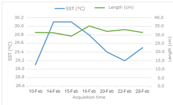
Figure 16. Relationship of SST and length of K. pelamis in February 2018
