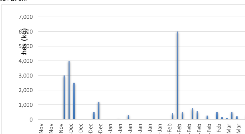
Figure 3. Daily catches in November, Desember, January, February, March 2018.
