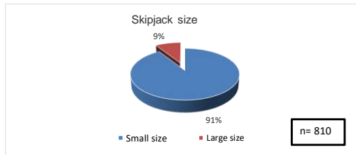
Figure 4. Katsuwonus pelamis size in November 2017-March 2018.
