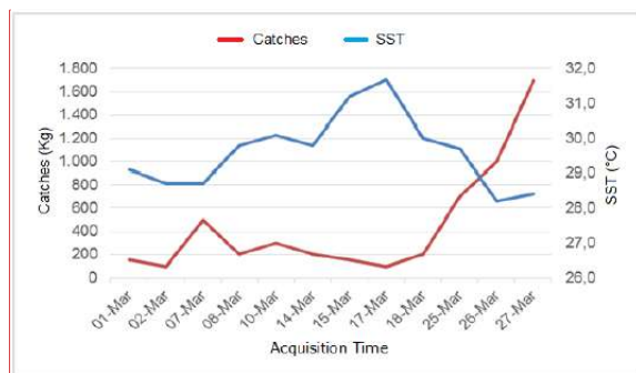
Figure 18. Relationship of SST and catches in March 2018 with a temperature range of 28.2-31.7°C with Katsuwonus pelamis catching range of 100-1,700 kg.
