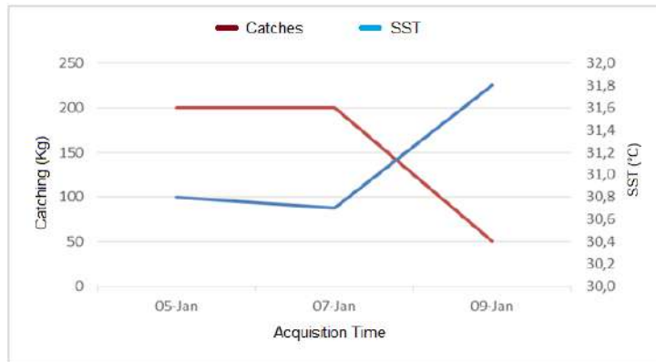
Figure 14. Relationship between SST and catch in January 2018 with a temperature range of 30.8°C to 31.8°C with catches of K. pelamis ranging from 50 kg to 200 kg.
