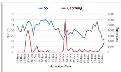
Figure 9. SST relationship with the catch of each setting.
