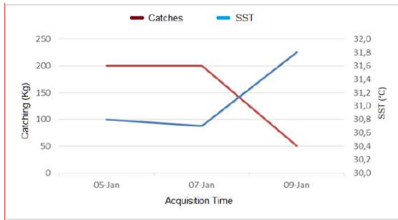
Figure 14. Relationship between SST and catch in January 2018 with a temperature range of 30.8-31.8°C with catches of Katsuwonus pelamis ranging from 50 to 200 kg.
