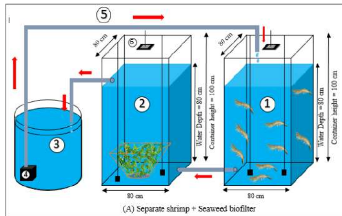
Figure 1. Biofilter system design (A).
