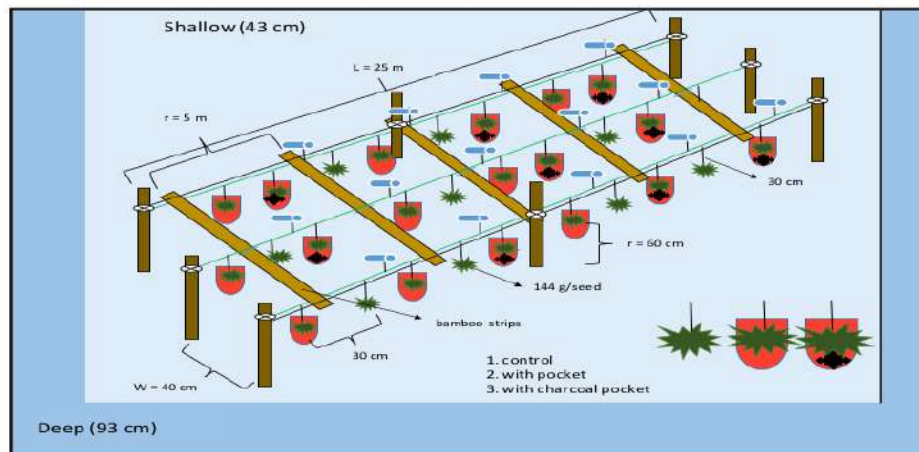
Figure 3. Intervention scheme of charcoal bag applications.
